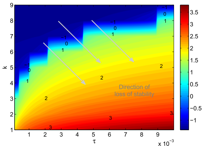
FIG. 3. Stability function over the set \tau \times k of the parameter space of a k -cycle network of 20 Rössler oscillators. 31 Note that sync stability is lost as the number of links decreases and the time-delay increases.
